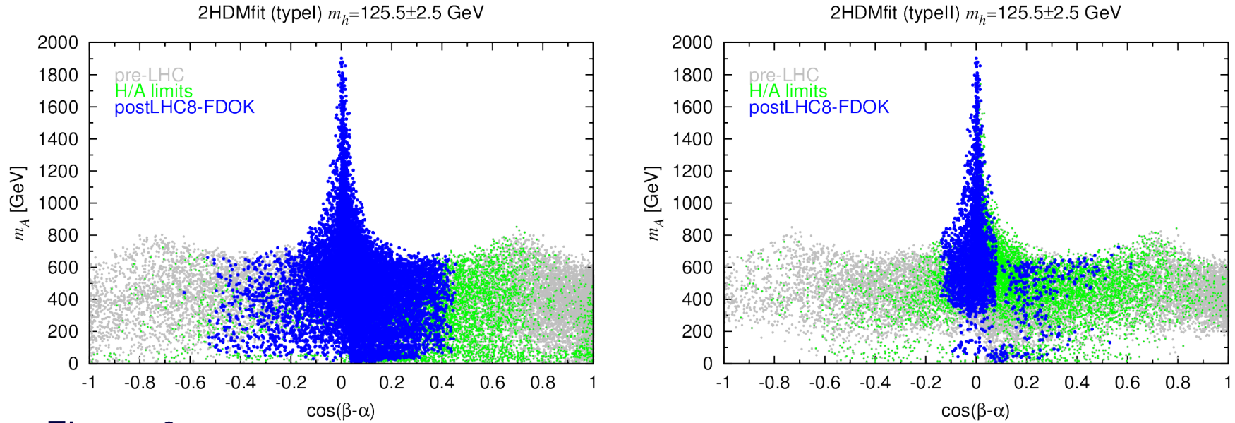
Figure 9: Constraints in the m_A versus \cos(\beta - \alpha) plane for m_h \sim 125.5 GeV.
