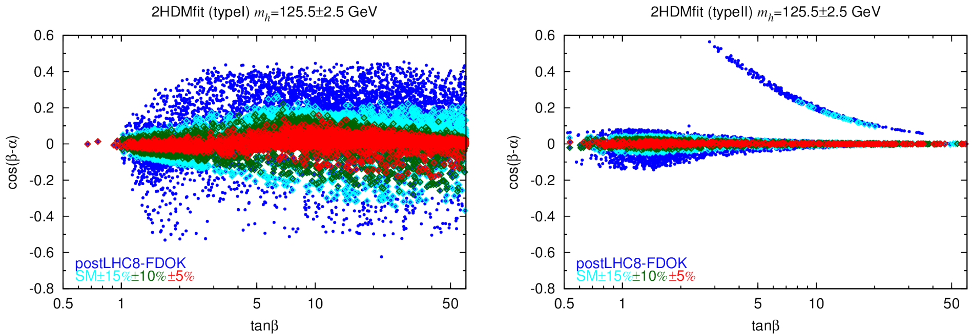
Figure 10: postLHC8-FDOK points in the \cos(\beta - \alpha) vs. \tan\beta plane for the m_h \sim 125.5 GeV scenario comparing current h fits (blue) to the case that all the channel rates are within \pm 15\% , \pm 10\% , \pm 5\% of the SM Higgs prediction.
